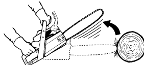
Kickback Path
